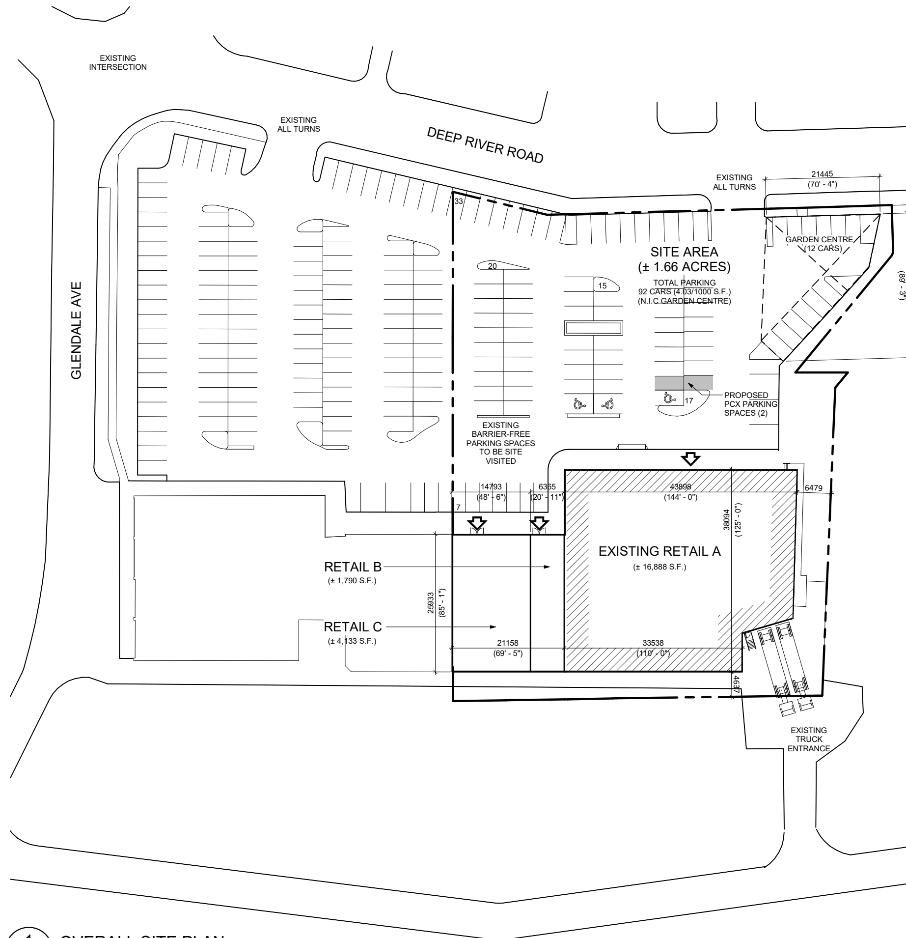
1 OVERALL SITE PLAN A1-24 1 : 700
